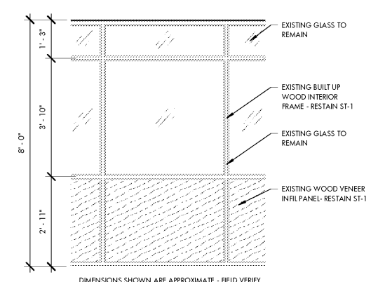
A3 EXISTING INTERIOR STOREFRONT ELEVATION TYP. A-602 1/2" = 1'-0"
