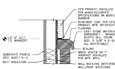
D WAINSCOT/STUCCO TRANSITION SCALE: 1 1/2" = 1'-0"
