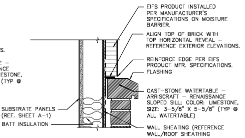
E BRICK/STUCCO TRANSITION @ MAIN ENTRY WALL SCALE: 1 1/2" = 1'-0"
