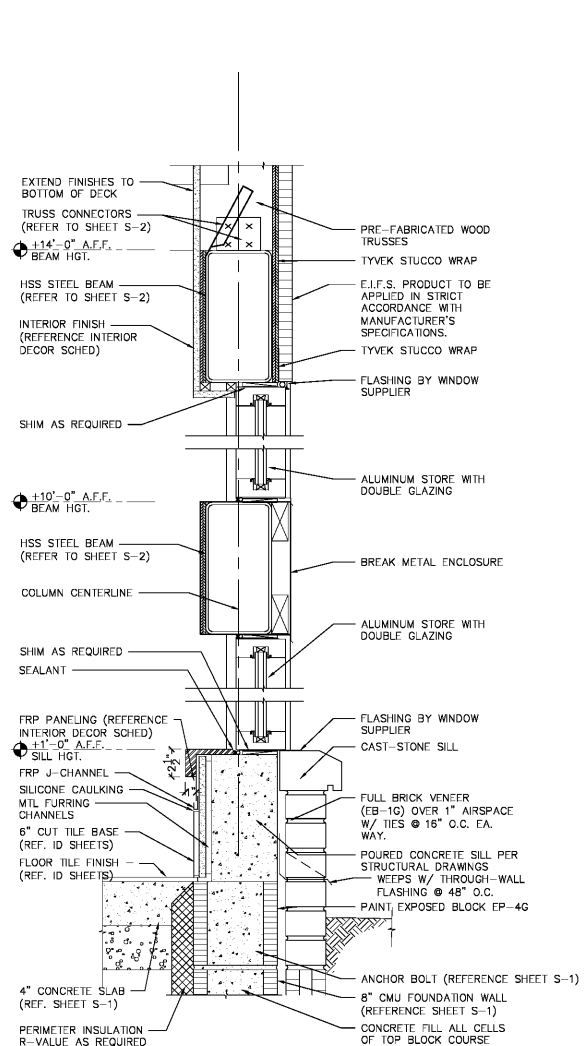
A BASE-SILL-HEADER-CAP DETAILS SCALE: 1-1/2" = 1'-0"
