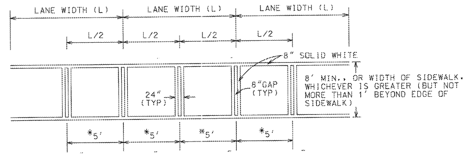
CROSSWALK DETAIL
