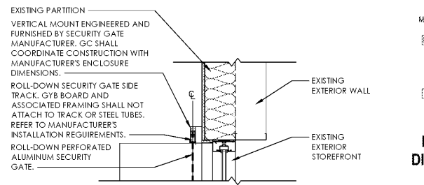
6 SECURITY GRILLE PLAN DETAIL @ JAMB BY OTHERS SCALE: 1" = 1'-0"
