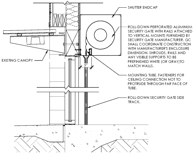
7 STOREFRONT SECTION - SECURITY GRILLE BY OTHERS SCALE: 1" = 1'-0"
