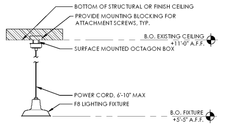
4 TYP. PENDANT LIGHT HANGING DETAIL SCALE: 1/2" = 1'-0"
