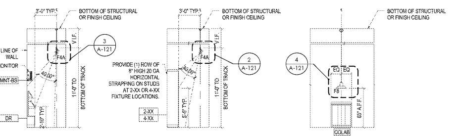
5 TYPICAL LIGHTING DETAILS - DIAGRAMS SCALE: NTS
