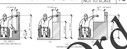
SIDE REACH
