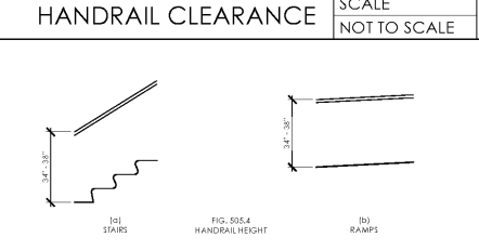
HANDRAILS
