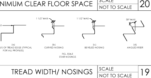
TREAD WIDTH/ NOSINGS
