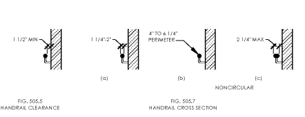
FIG. 505.6 HANDRAIL CLEARANCE
