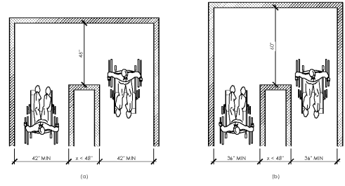
FIG. 403.5.1 CLEAR WIDTH AT 180° TURN
