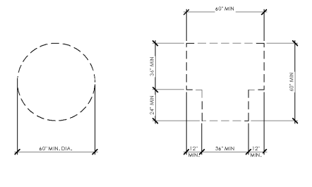
FIG. 504.3 SIZE OF TURNING SPACE
