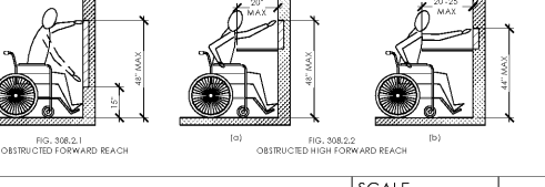
FORWARD REACH
