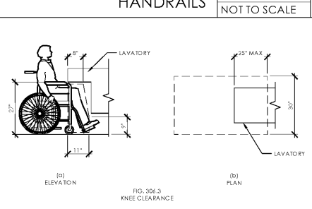
LAVATORY KNEE & TOE CLEARANCES
