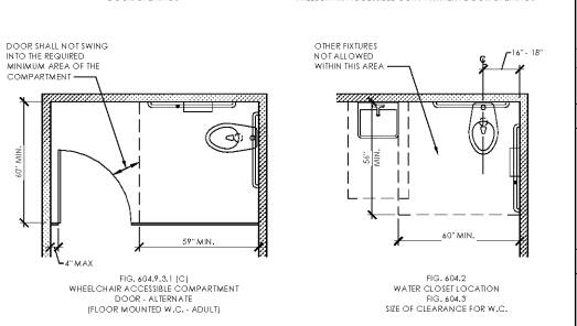
WATER CLOSET & TOILET COMPARTMENT
