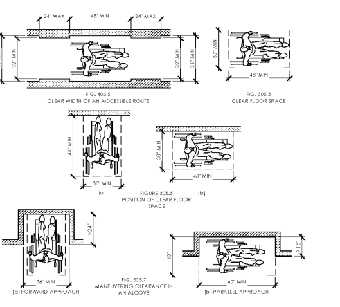
MINIMUM CLEAR FLOOR SPACE
