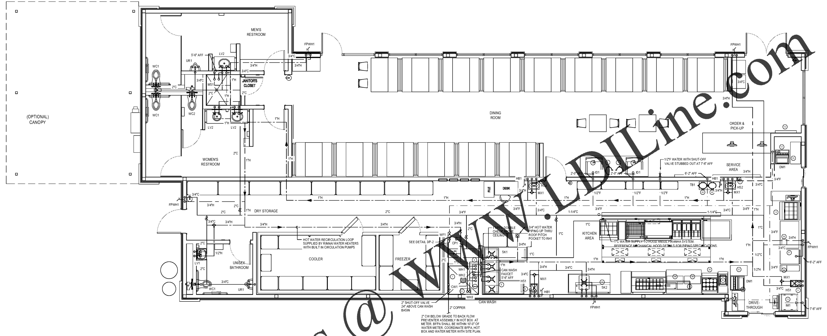
1 WATER PIPING PLAN P-5 SCALE: 1/4" = 1'-0"
