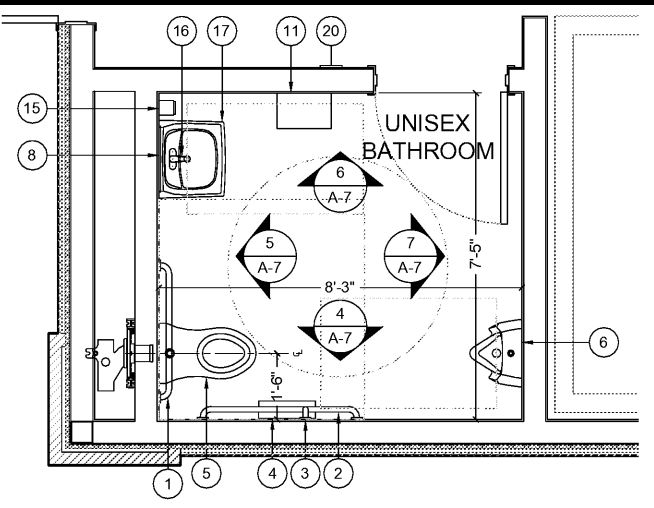
2 UNISEX / EMPLOYEE RESTROOM ACCESSORY PLAN SCALE: 1/2" = 1'-0"
