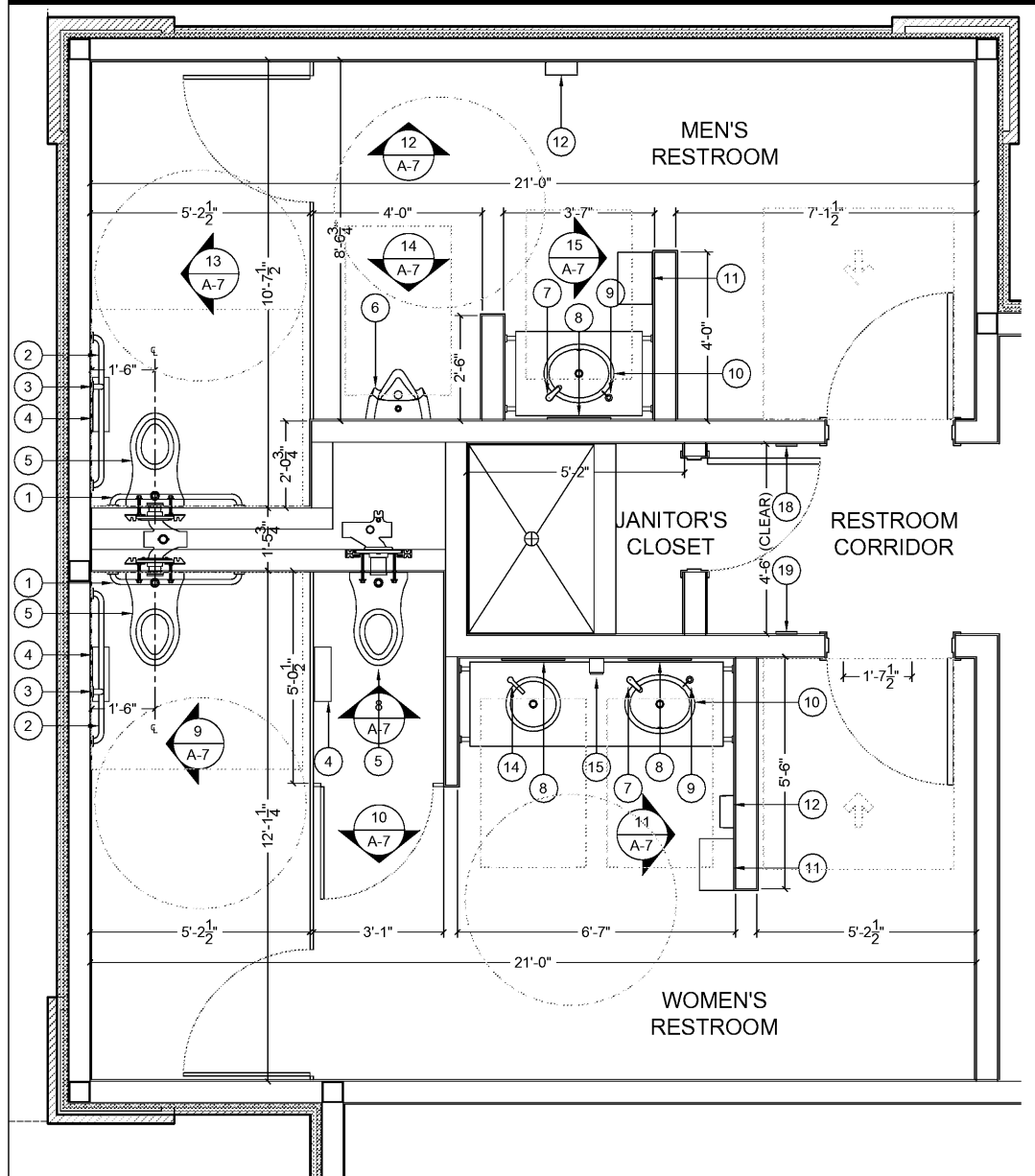
1 MEN'S & WOMEN'S RESTROOM ACCESSORY PLAN SCALE: 1/2" = 1'-0"
