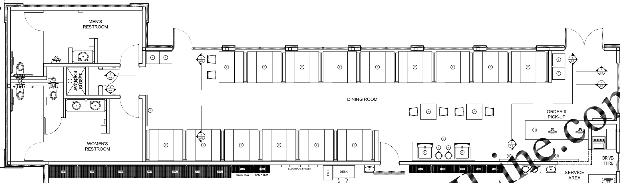
1 FURNITURE FLOOR PLAN A-6 SCALE: 1/4" = 1'-0"
