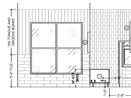
3 DINING ROOM A-6 SCALE: 1/4" = 1'-0"
