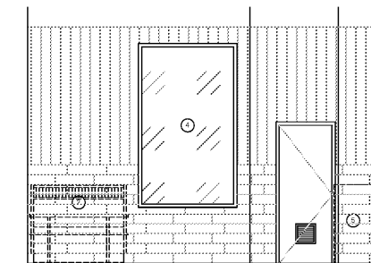
5 DINING ROOM A-6 SCALE: 1/4" = 1'-0"
