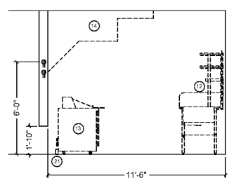
5 KITCHEN HOOD A-5 SCALE: 1/4" = 1'-0"
