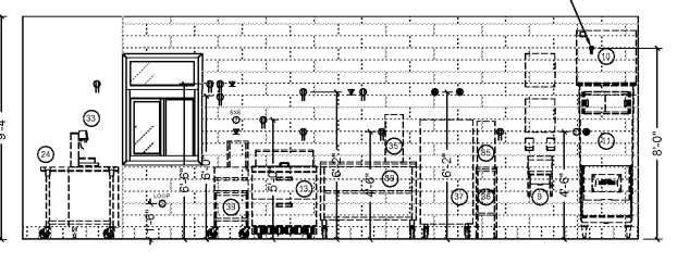
4 KITCHEN SERVICE AREA A-5 SCALE: 1/4" = 1'-0"
