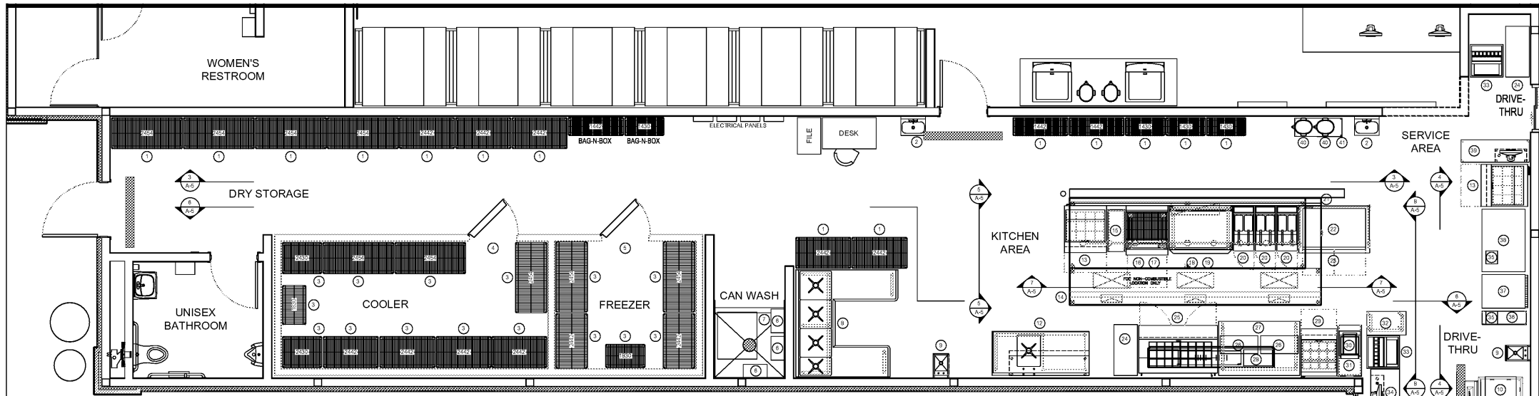
1 EQUIPMENT FLOOR PLAN A-5 SCALE: 1/4" = 1'-0"
