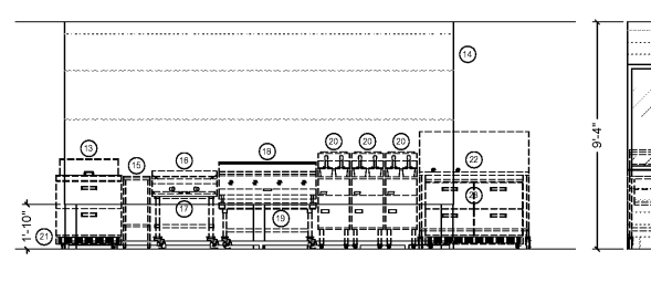
7 KITCHEN HOOD A-5 SCALE: 1/4" = 1'-0"
