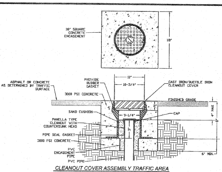
CLEANOUT COVER ASSEMBLY TRAFFIC AREA
