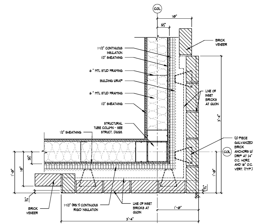
5 DETAIL @ PILASTERS SCALE: 1 1/2"=1'-0"
