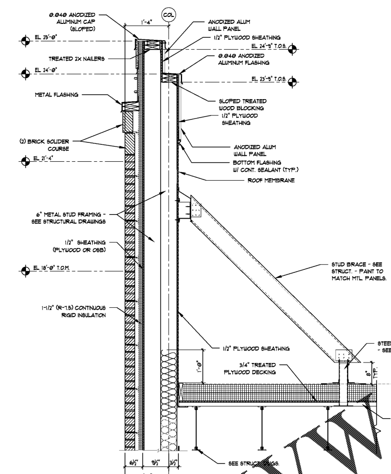
2 COPING DETAIL AT STEPPED WALL SCALE: 3/4"=1'-0"
