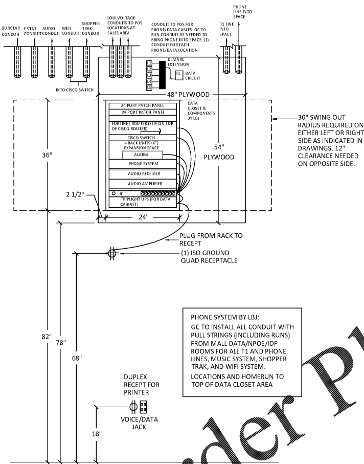
1 DATA CABINET ELEVATION E3 SCALE: NONE
