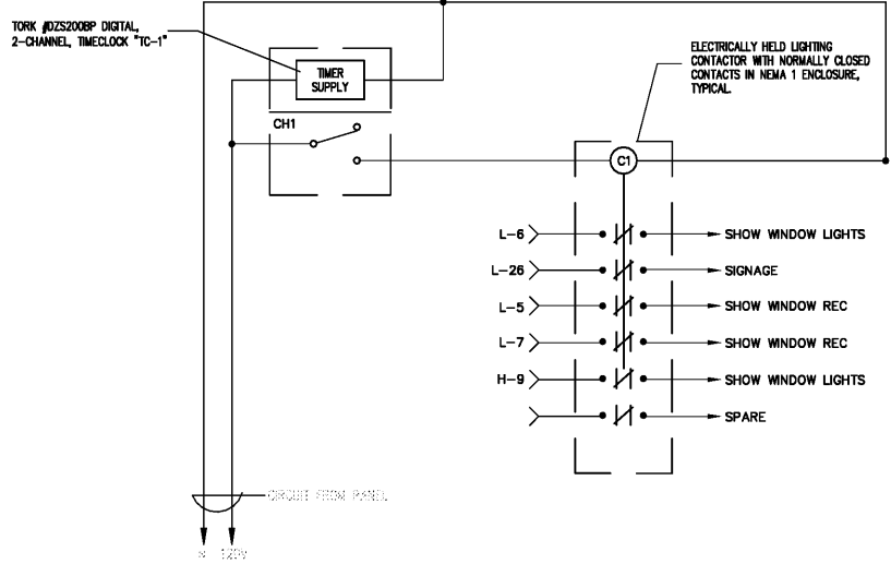
3 TIME CLOCK DETAIL E3 SCALE: NONE
