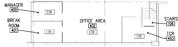
6E REFLECTED CEILING PLAN - ELEVATED OFFICE SCALE: 3/32" = 1'-0"
