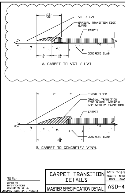
TRANSITION DETAILS MASTER SPECIFICATION DETAIL DATE: 7/13/16 SCALE: NONE DRAWN: ZAV ASD-4B
