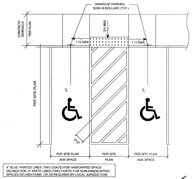
ADA PARKING LAYOUT DETAIL NOT TO SCALE
