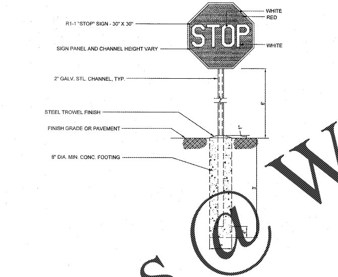
TRAFFIC SIGN MOUNTING DETAIL NOT TO SCALE
