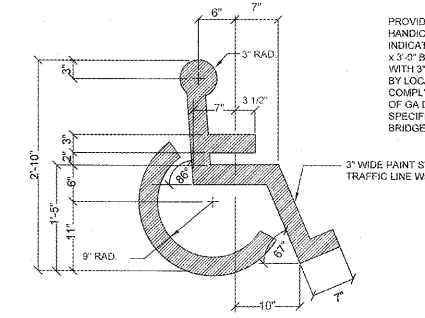
ADA PARKING SYMBOL DETAIL NOT TO SCALE
