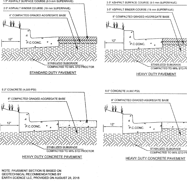
PAVEMENT SECTION DETAIL NOT TO SCALE
