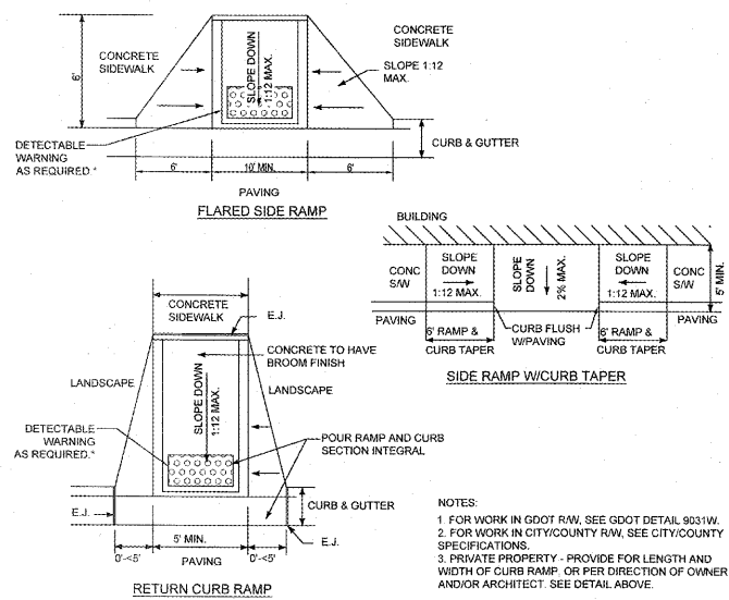
ADA PARKING RAMP DETAIL NOT TO SCALE
