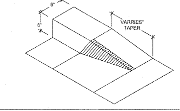
TAPER CURB DETAIL NOT TO SCALE
