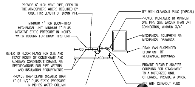
PIPING ARRANGEMENT SHOWN IS SCHEMATIC. ADJUST AS REQUIRED TO SUIT ACTUAL INSTALLATION CONDITIONS. REFER TO ALL CODES FOR INDIRECT DRAIN REQUIREMENTS. 3 AIR HANDLING UNIT CONDENSATE DRAIN NOT TO SCALE
