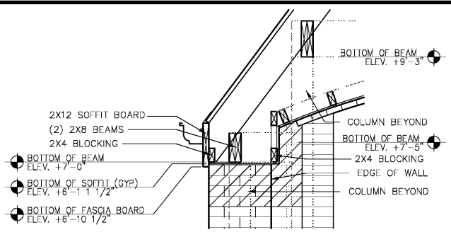
5 SECTION DETAIL SCALE: 3/4" = 1'-0"
