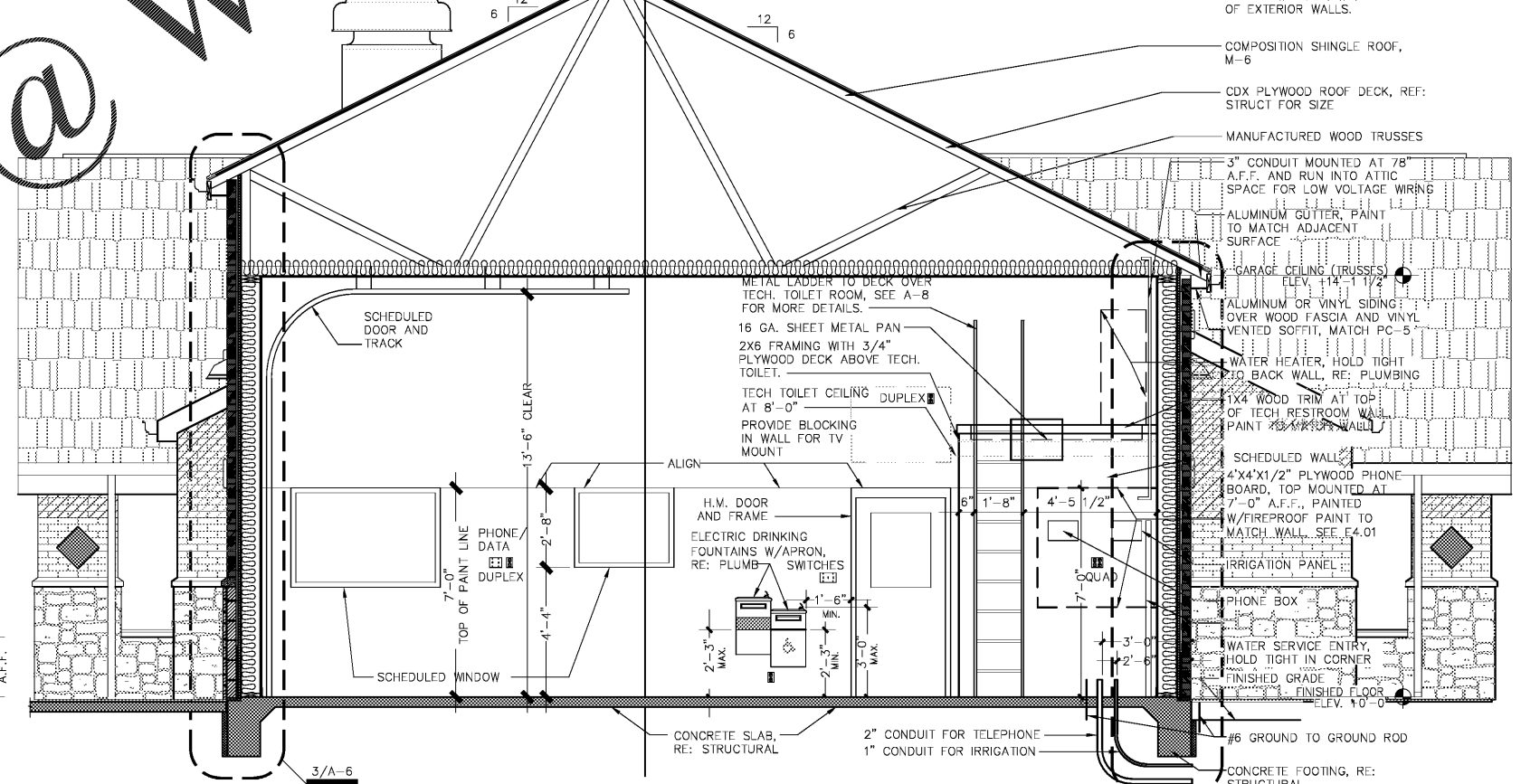
1 BUILDING SECTION SCALE: 3/8" = 1'-0"
