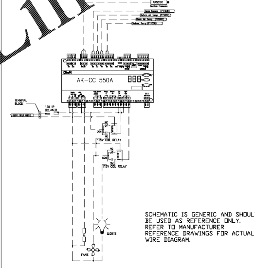
2 CC2 SAMPLE SCHEMATIC CASE & WALK-IN W/O ELECTRIC DEFROST SCALE: NONE
