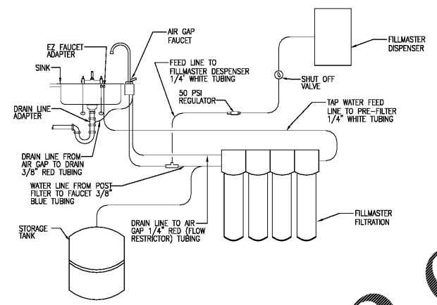
R87 WATER PURIFICATION AND DISPENSING SYSTEM @ PHARMACY NOT TO SCALE
