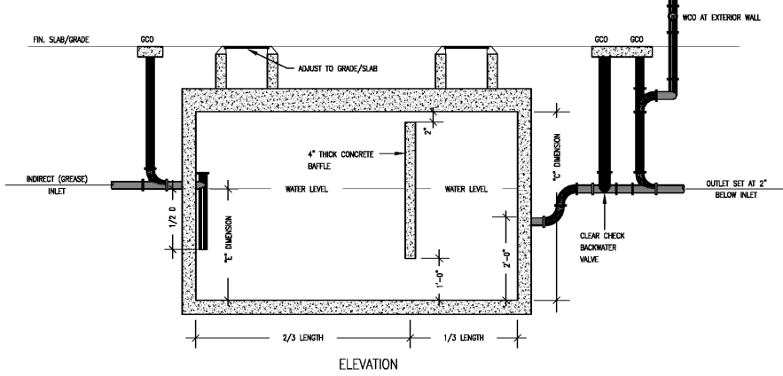
3000 GALLON GREASE BASIN DETAIL NOT TO SCALE
