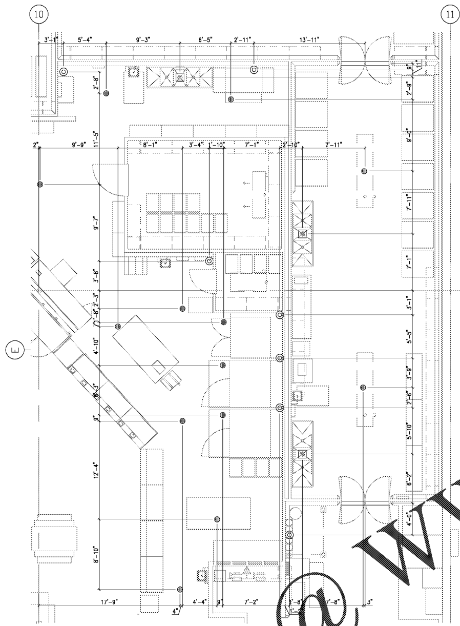
01 ENLARGED PLUMBING DIMENSION PLAN SCALE: 1/4" = 1'-0"
