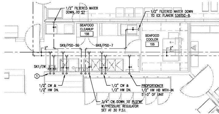
02 ENLARGED WATER PLAN SCALE: 1/4" = 1'-0"
