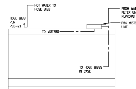
5-DECK PRODUCE CASE elevation DETAIL 'A'
