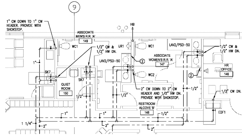
01 ENLARGED WATER PLAN SCALE: 1/4" = 1'-0"
