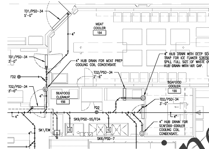
03 ENLARGED WASTE AND VENT PLAN SCALE: 1/4" = 1'-0"
