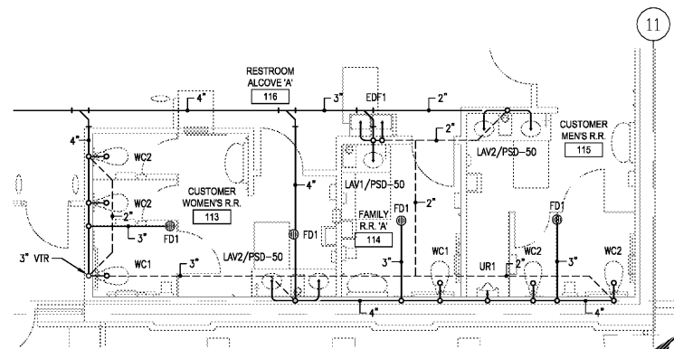
02 ENLARGED WASTE AND VENT PLAN SCALE: 1/4" = 1'-0"
