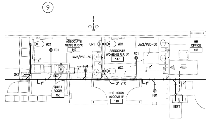
01 ENLARGED WASTE AND VENT PLAN SCALE: 1/4" = 1'-0"
