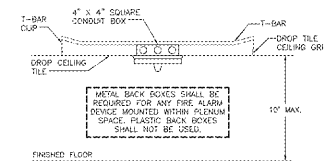
CEILING HORN/STROBE FLUSH MOUNTING DETAIL SCALE: NO SCALE
