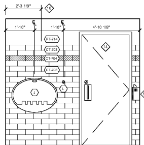
FAMILY RESTROOM 'C' #187 11 #RESTROOM ELEVATIONS
