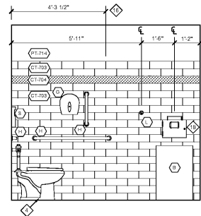
ASSOCIATE MEN'S 'B' #168 01 #RESTROOM ELEVATIONS
