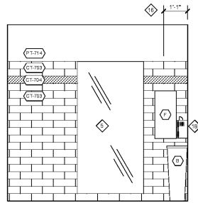
ASSOCIATE WOMEN'S 'B' #169 04 #RESTROOM ELEVATIONS
