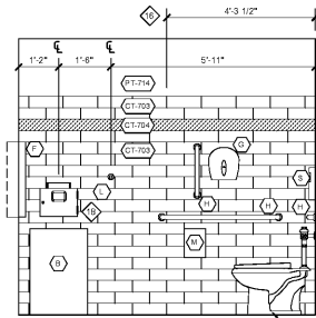
ASSOCIATE WOMEN'S 'B' #169 05 #RESTROOM ELEVATIONS
