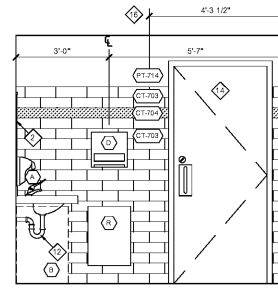
ASSOCIATE WOMEN'S 'B' #169 03 #RESTROOM ELEVATIONS
