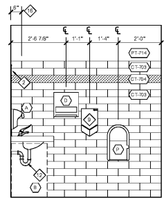
FAMILY RESTROOM 'B' #186 FAMILY RESTROOM 'C' #186 07 #RESTROOM ELEVATIONS
