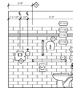
FAMILY RESTROOM 'B' #186 FAMILY RESTROOM 'C' #186 09 #RESTROOM ELEVATIONS
