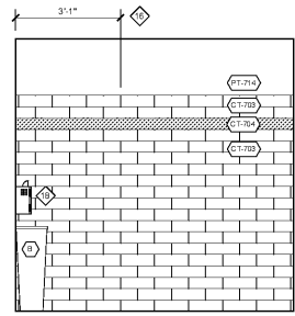
ASSOCIATE MEN'S 'B' #168 02 #RESTROOM ELEVATIONS
