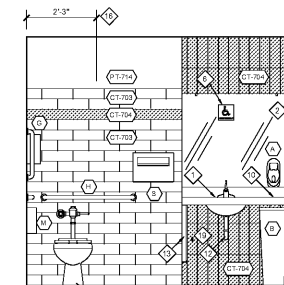
FAMILY RESTROOM 'C' #187 12 #RESTROOM ELEVATIONS
