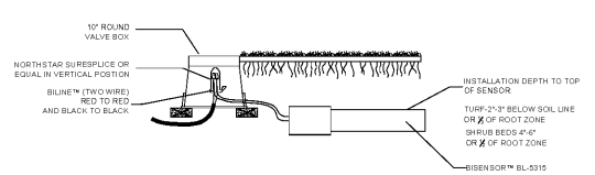
9 MOISTURE SENSOR PLACEMENT
