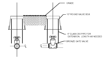
10 ISOLATION VALVE DETAIL
