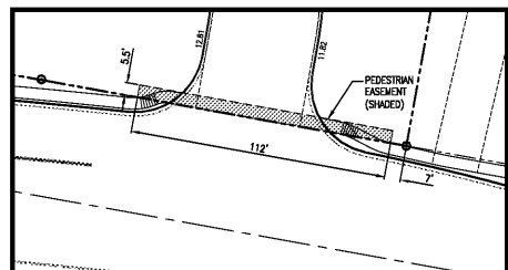
PEDESTRIAN EASEMENT LAYOUT SCALE: 1" = 30'
