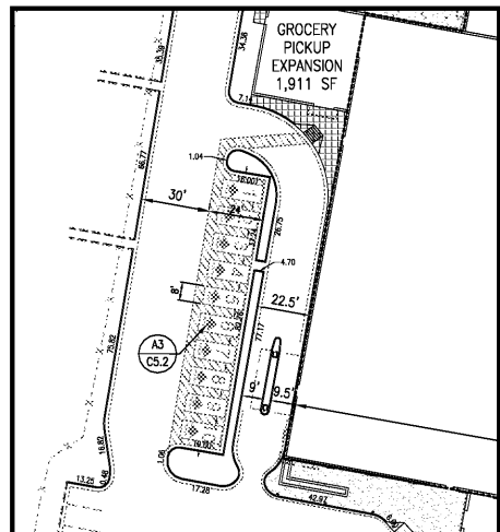
GROCERY PICK UP PARKING LAYOUT SCALE: 1" = 30'
