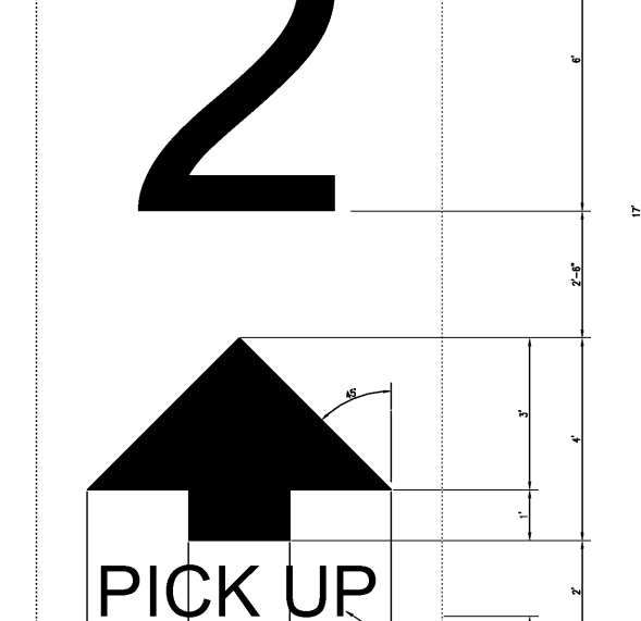
3A PHARMACY DRIVE-THRU NOT TO SCALE 4A GROCERY PICK UP INFORMATIONAL SIGN NOT TO SCALE
