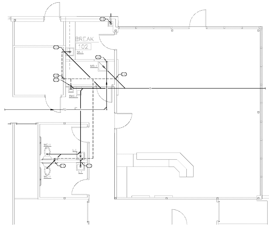
3 ENLARGED PLAN - WASTE & VENT SCALE: 1/4"=1'-0"
