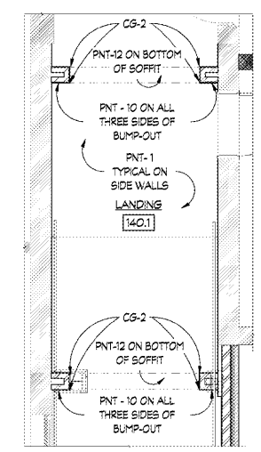
4 TYPICAL ENLARGED LANDING FINISH DETAIL SCALE: 1/4" = 1'-0"
