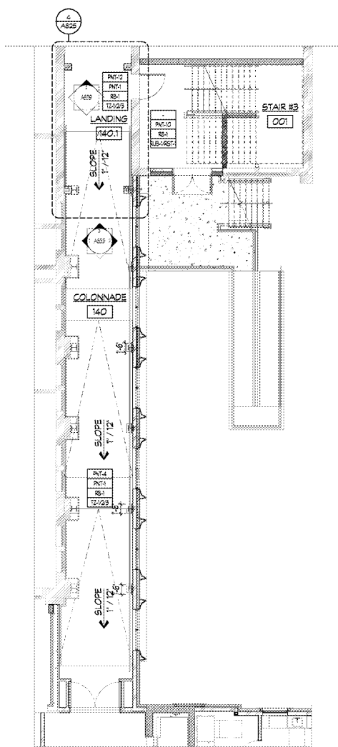
1 FIRST FLOOR COLONNADE FINISH PLAN SCALE: 1/8" = 1'-0"
