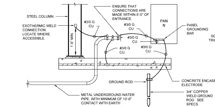
2 ELECTRODE GROUNDING DETAIL E-401 SCALE: NOT TO SCALE
