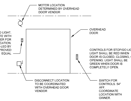
3 OVERHEAD DOOR DETAIL EQUIPMENT LOCATIONS E-401 SCALE: NONE
