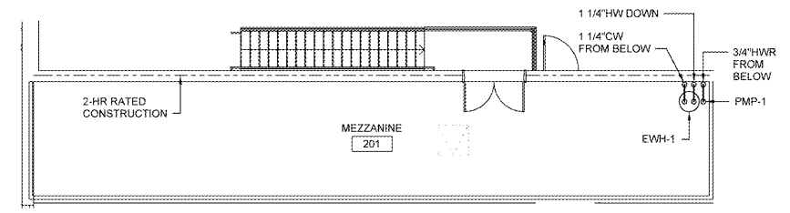
② MEZZANINE POTABLE WATER PIPING PLAN SCALE: 1/8" = 1'-0"
