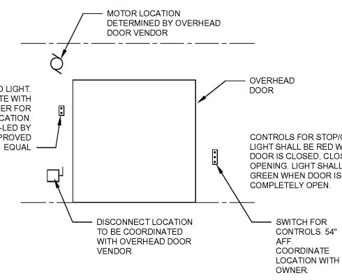
3 OVERHEAD DOOR DETAIL EQUIPMENT LOCATIONS SCALE: NONE
