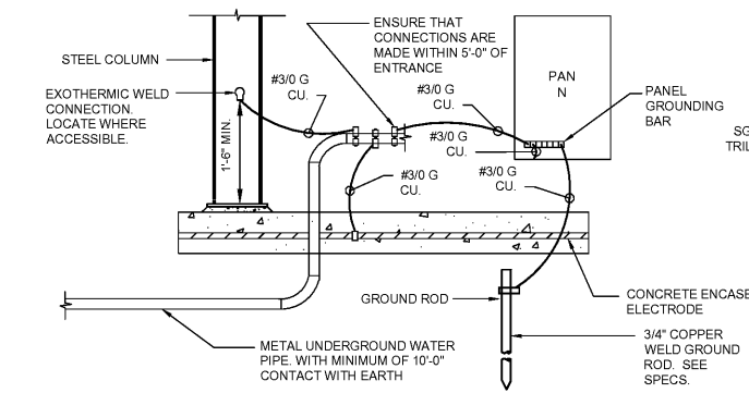
2 ELECTRODE GROUNDING DETAIL SCALE: NOT TO SCALE
