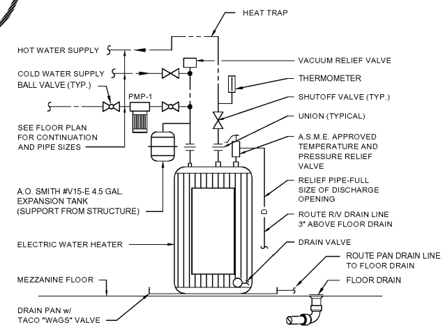
(EWH-1) SCHEMATIC - ELECTRIC WATER HEATER NO SCALE
