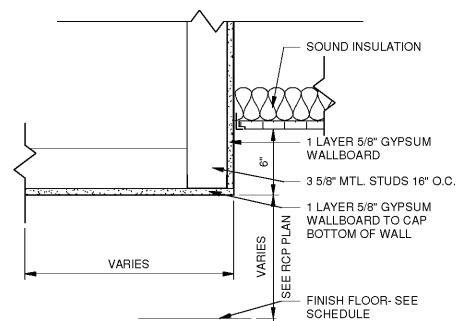
3 A-201 BULKHEAD DETAIL SCALE: 1 1/2" = 1'-0"
