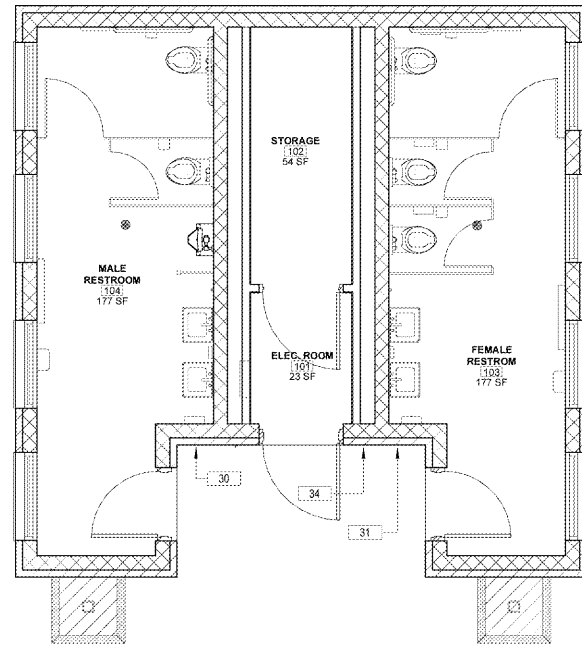
1 FINISH PLAN & SIGNAGE PLAN A701 1/4" = 1'-0"
