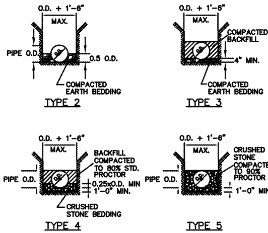
TYPICAL PIPE BEDDING DETAILS
