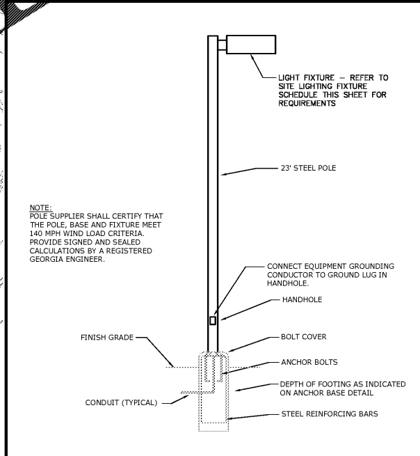
POLE DETAIL-TYPICAL NOT TO SCALE
