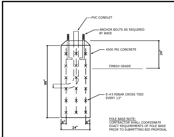
POLE ANCHOR BASE DETAIL NOT TO SCALE
