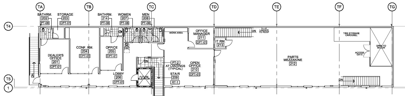
PROPOSED SECOND FLOOR FINISH PLAN 3/32"=1'-0" SECOND FLOOR BUILDING AREA: 4986 S.F. NOTE: THIS BUILDING IS EQUIPPED WITH AN AUTOMATIC SPRINKLER SYSTEM.
