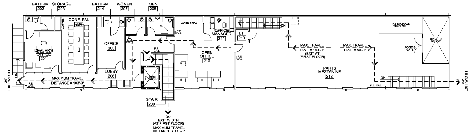
1 A0.2 SECOND FLOOR LIFE SAFETY PLAN 3/32"=1'-0" SECOND FLOOR BUILDING AREA: 4986 S.F. NOTE: THIS BUILDING IS EQUIPPED WITH AN AUTOMATIC SPRINKLER SYSTEM.
