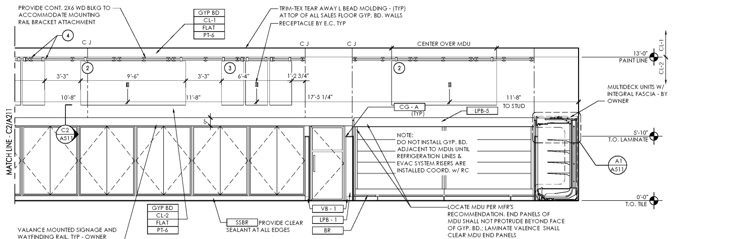
Retail Interior Elevation B1 SCALE: 1/4" = 1'-0"
