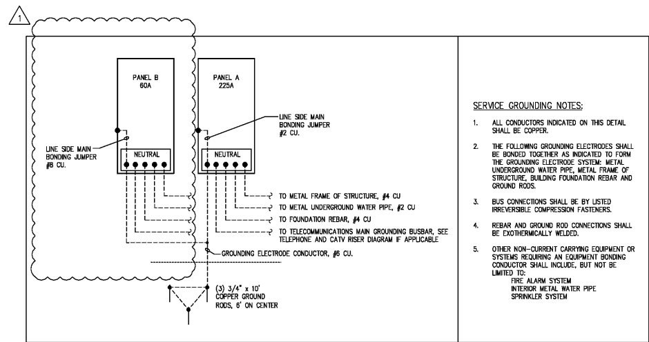
SERVICE GROUNDING DIAGRAM SCALE: NONE
