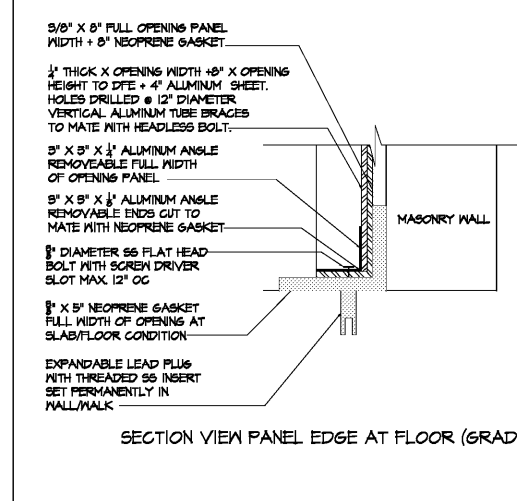
13 FLOOD PANELS DETAILS SCALE: 3" = 1'-0"
