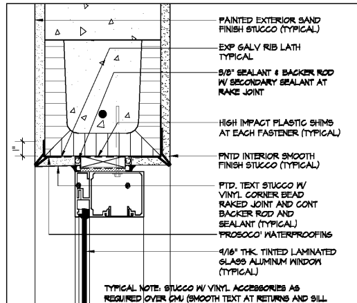
5 FIXED WINDOW HEAD SCALE: 3" = 1'-0"
