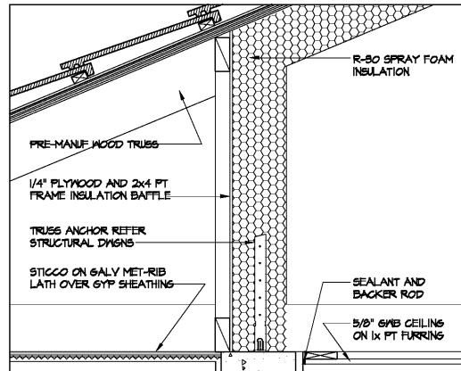
2 TRUSS INSULATION BATTLE SCALE: 1 1/2" = 1'-0"
