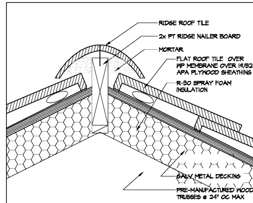
3 RIDGE VENT DETAIL SCALE: 3" = 1'-0"
