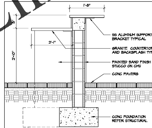
15 OUTDOOR BAR SCALE: 3/4" = 1'-0"
