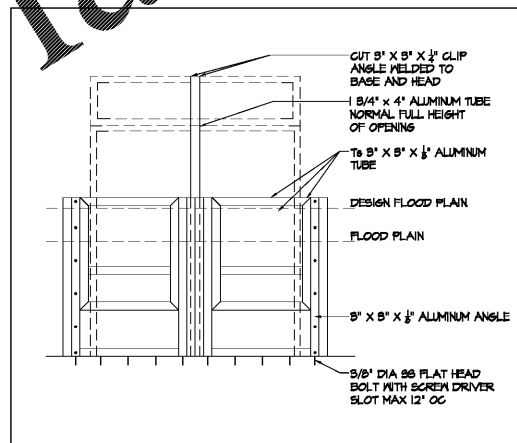
12 FLOOD PANELS ELEVATION SCALE: 3/8" = 1'-0"
