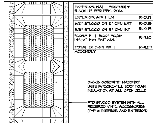
4 TYPICAL EXTERIOR WALL SCALE: 3" = 1'-0"
