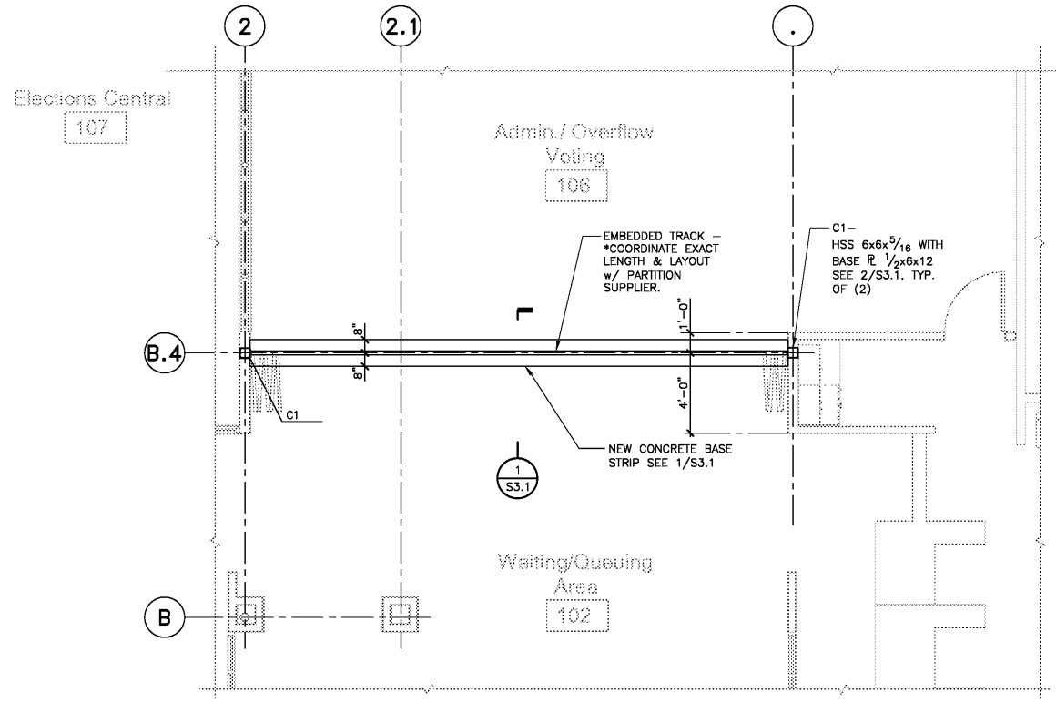
OPERABLE PARTITION FLOOR PLAN SCALE: 1/4" = 1'-0" (1) S2.1
