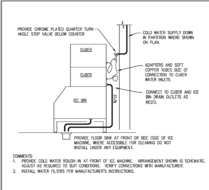
2 ICE MACHINE PIPING SCHEMATIC
