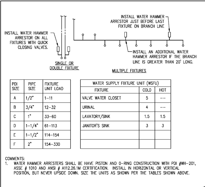
3 WATER HAMMER ARRESTER DETAIL
