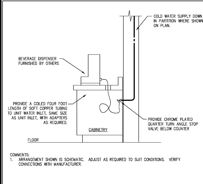
1 BEVERAGE WATER PIPING SCHEMATIC
