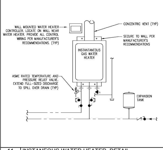
11 INSTANEOUS WATER HEATER DETAIL
