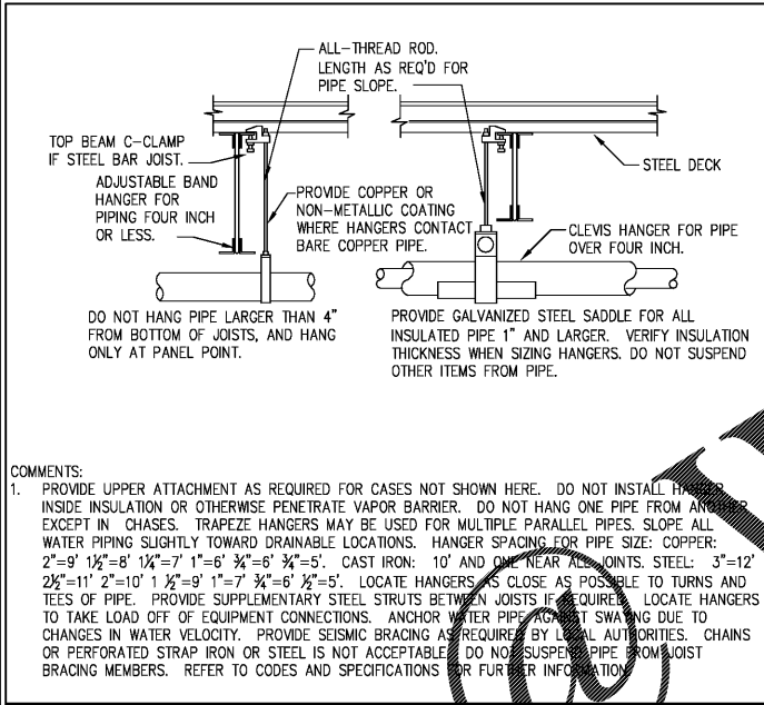
6 PIPE HANGER DETAIL
