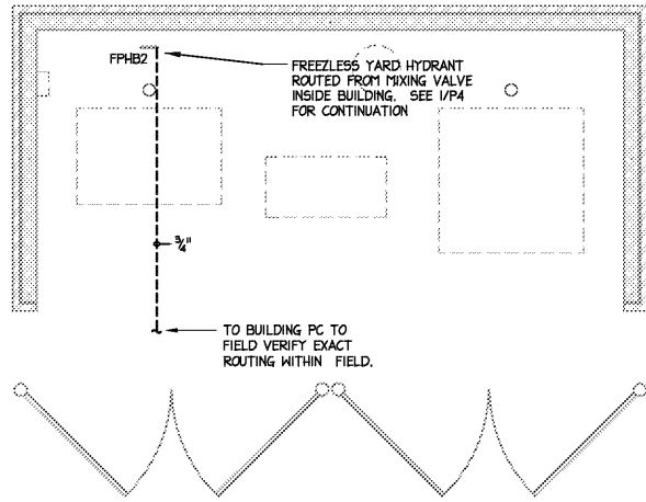
2 WASTE ENCLOSURE WATER PLAN 1/4"=1'-0"
