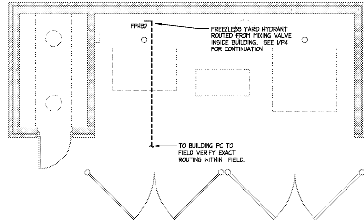
3 WASTE ENCLOSURE W/STORAGE WATERPLAN 1/4"=1'-0"
