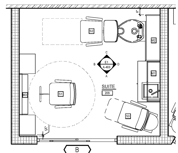
A12 Typical Enlarged Suite Plan SCALE: 1/2" = 1'-0"
