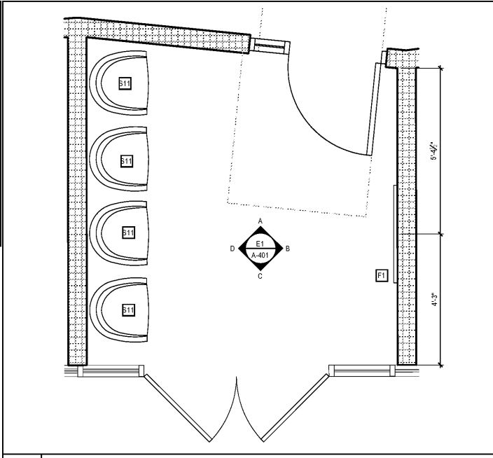
A12 Enlarged Lobby Plan SCALE: 1/2" = 1'-0"
