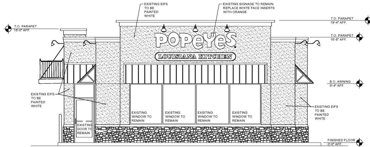
1 FRONT ELEVATION A5 1/4"=1'-0"
