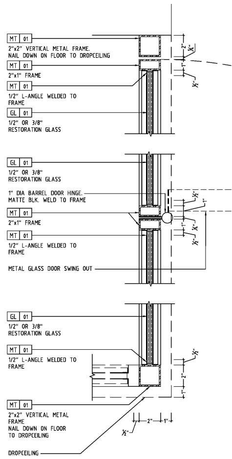
1 FRONT COUNTER DETAIL A4.2 3'-1'-0"
