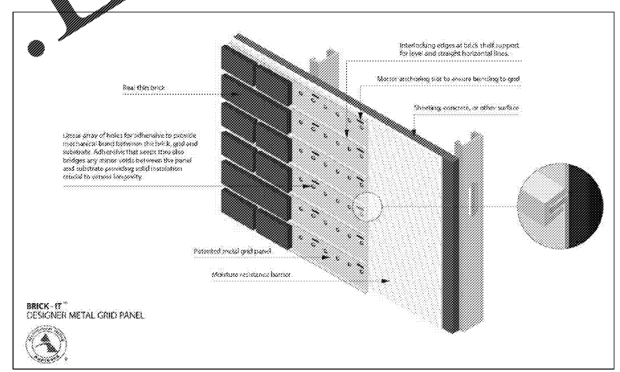
3 TYP. THIN BRICK VENEER SYSTEM A5 NTS
